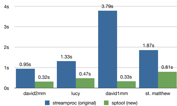
Figure 4: Comparison of average time each point spends in main memory.
