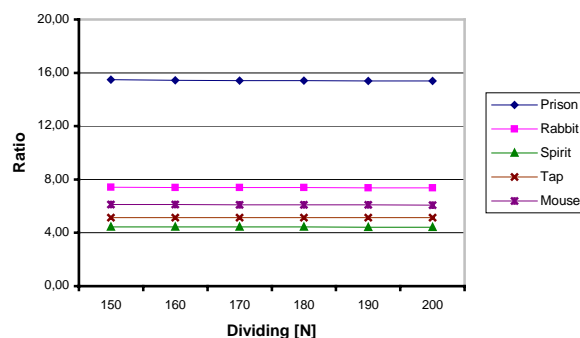
Figure 10. Speed-up ratio (Microsoft Visual C++).
