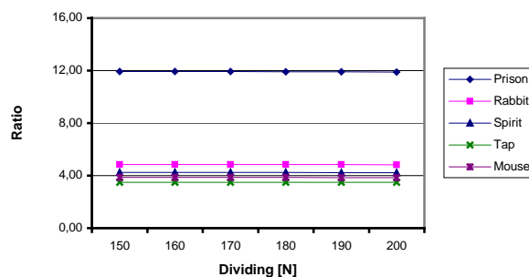
Figure 11. Speed-up ratio (Borland C++ Builder).
