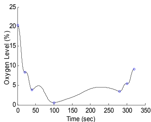
Figure 1. Graph through the data in Table 1 using the Shepard's method
