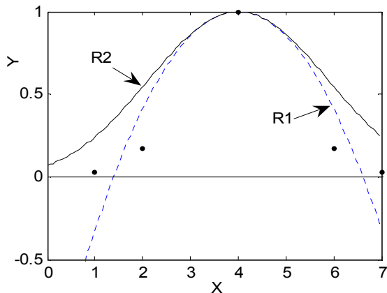
Figure 4. The quadratic basis function (R1) has values less than 0 while the constrained basis function (R2) remains above 0.
