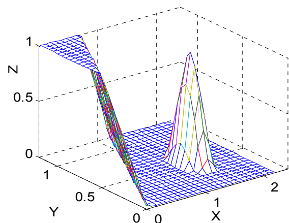
Figure 8. Test function (18) plotted at 25x25 grids.
