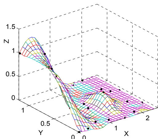
Figure 6. A randomly generated dataset (N=30) using the test function (18) is plotted using the MQS method. The graph does not preserve [0, 1] bounds of data.
