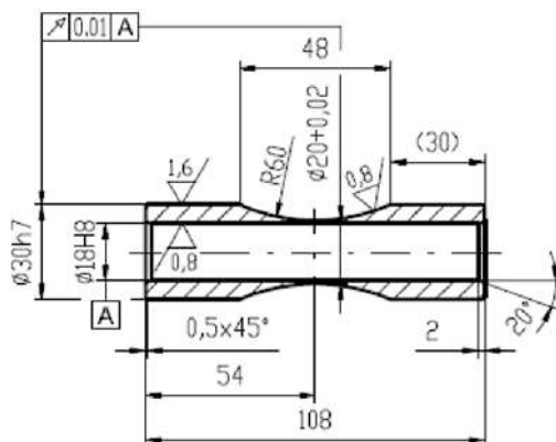
Fig. 1. Testing specimen
