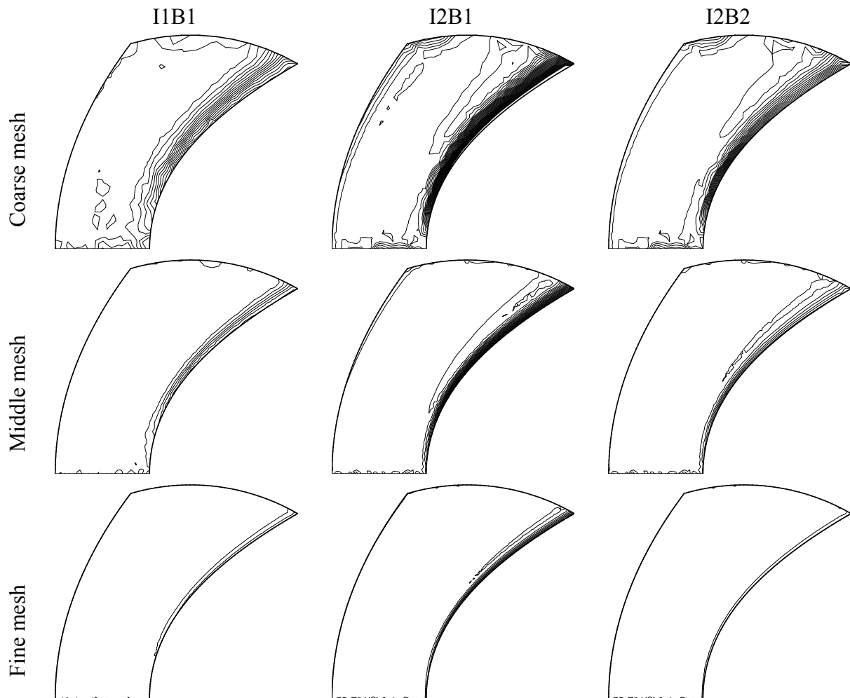
Fig. 3. Isolines of the entropy for the Ringleb's flow, three different interpolations (columns) and three levels of meshes (rows).
