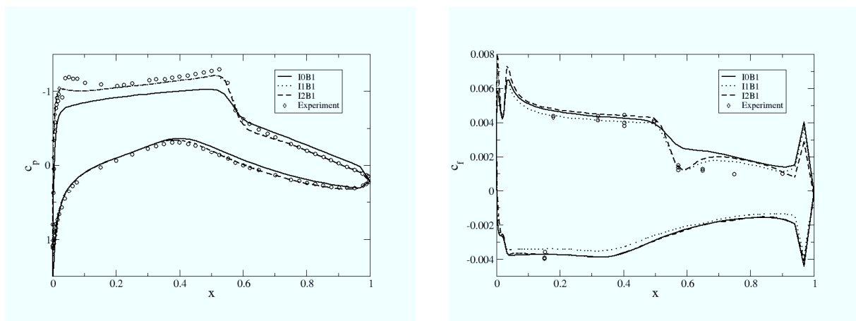
Fig. 7. Distribution of pressure and friction coefficients obtained with the low order (I0B1), the second order (I1B1), and the mixed order (I2B1) schemes.
