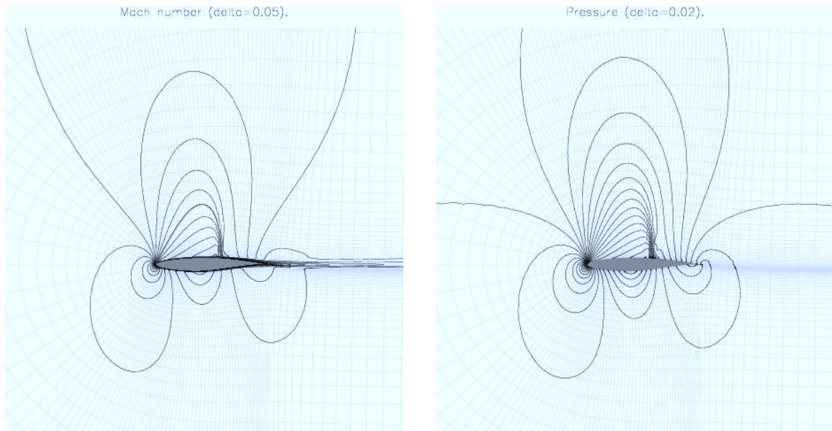
Fig. 6. Isolines of the Mach number and the pressure for the flow around the RAE 2822 profile obtained with the mixed order scheme (I2B1) M_\infty = 0.73 , \alpha_\infty = 2.79^\circ , Re = 6.5 \cdot 10^6 .
