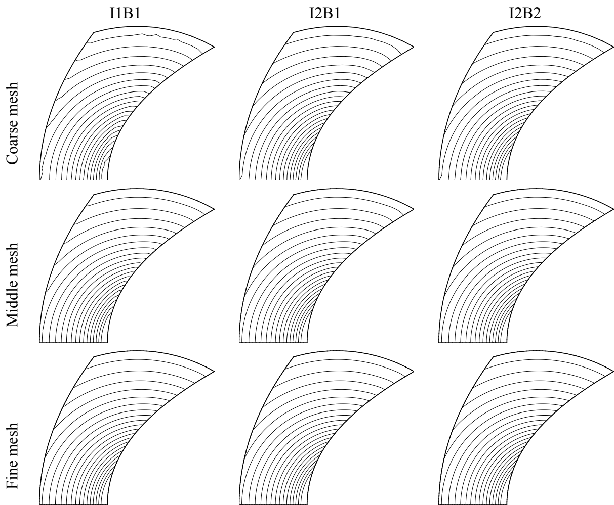
Fig. 2. Isolines of the Mach number for the Ringleb's flow, three different interpolations (columns) and three levels of meshes (rows).
