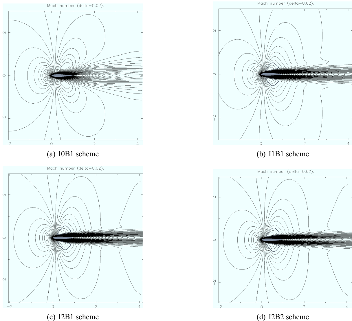
Fig. 4. Isolines of the Mach number for the laminar flow over NACA 0012 profile.
