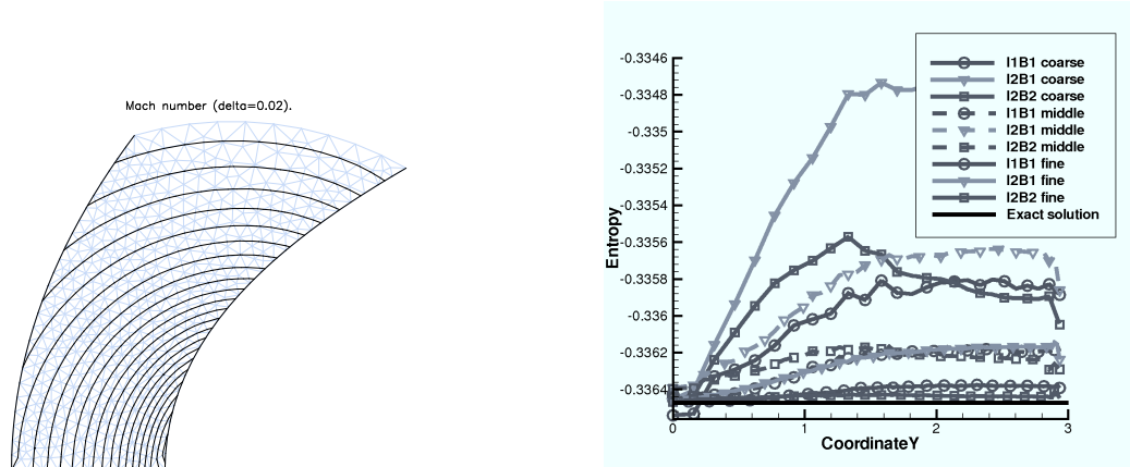
Fig. 1. Isolines of the Mach number and distribution of the entropy along the left wall for Ringleb's flow problem.
