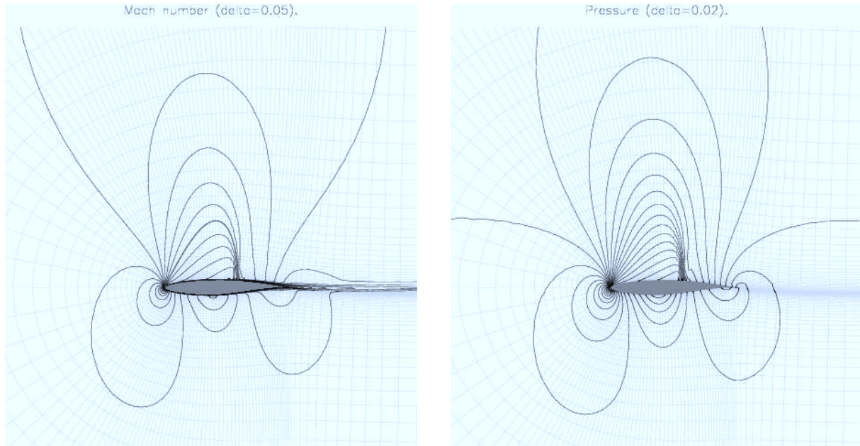
Fig. 5. Isolines of the Mach number and the pressure for the flow around the RAE 2822 profile obtained with the second order scheme (I1B1), M_\infty = 0.73 , \alpha_\infty = 2.79^\circ , Re = 6.5 \cdot 10^6 .
