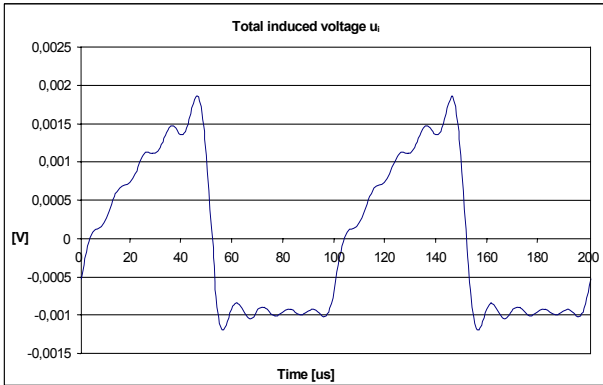
Fig. 7: Calculated course of total induced voltage u_i inside the investigated loop
