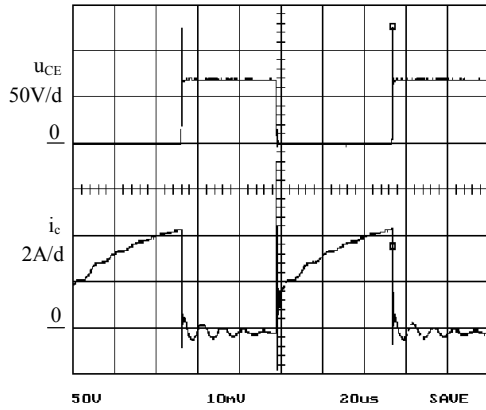
Fig. 3: Measured transistor current and voltage
