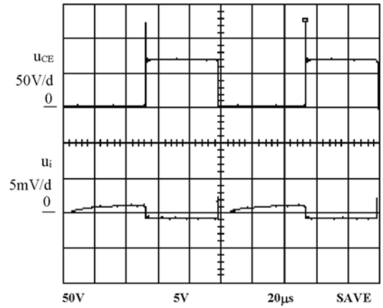
Fig. 8: Measured course of total induced voltage u_i
