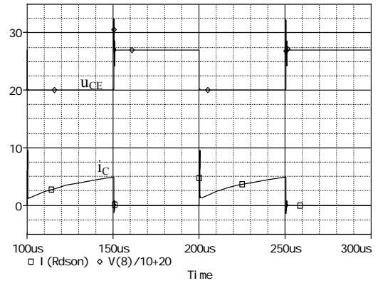
Fig. 2: Transistor voltage and current obtained by simulation
