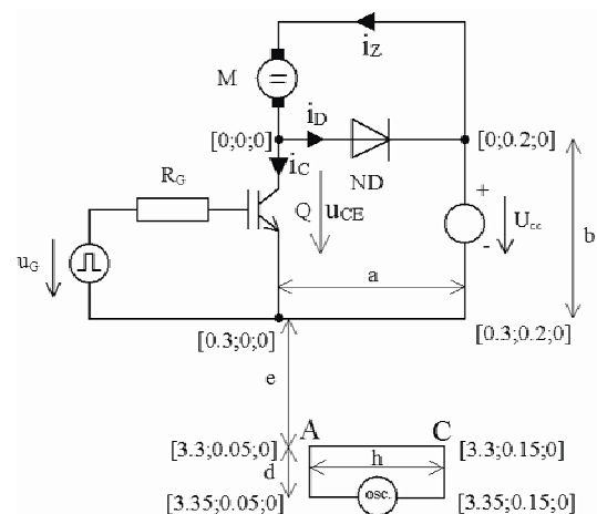
Fig. 1: Investigated circuit scheme
