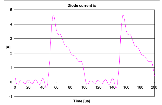
Fig. 5: Diode current - synthesis by 9 members of Fourier series
