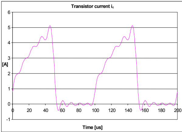
Fig. 4: Transistor current - synthesis by 9 members of Fourier series
