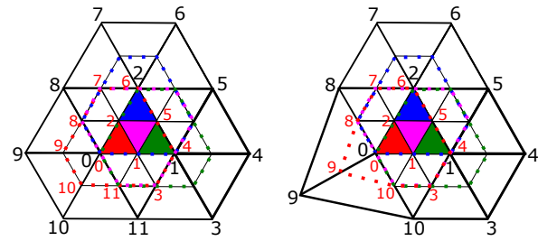
Figure 10: Patches and subpatches of the Loop subdivision scheme for the regular case (valence 6) and an irregular case (valence 5). Notice that the red subpatch is connectively-identical to the parent one and the other three are regular.
