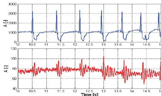
Figure 7. ACC method. ECG raw signal (top) and raw signal form accelerometer (bottom)
