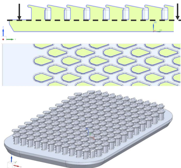
Figure 2. The 1st design iteration of cooling body, horizontal plane section is placed under overset faces
