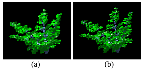
Renderings of a fern model, (a) LDI; (b) LRT. Figure 3
