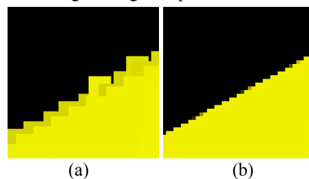
Zoomed-in edge of a cube rendered with (a) LDIs (b) LRTs Figure 5
