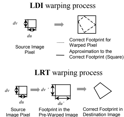
Approximation of Splat Shape Figure 2
