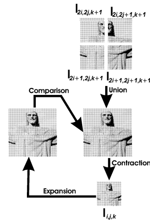
Figure 2: Construction method of the multi-resolution structure.
