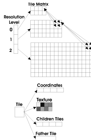
Figure 4: Multi-resolution data structure.
