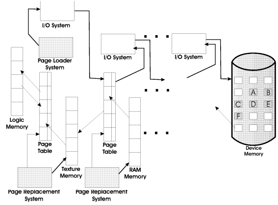
Figure 7: The predictive paging mechanism structure.
