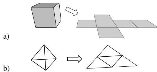
Figure 3. Unraveling the cube (a) and the tetrahedron (b).
