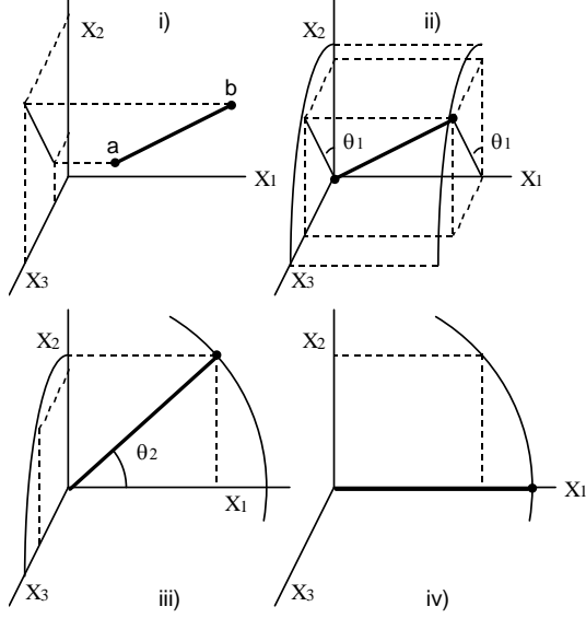
Figure 1. Set of transformations needed to align segment S = \overline{\mathbf{ab}} to axis X_1 .
