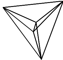
Figure 2. The 4D Simplex.
